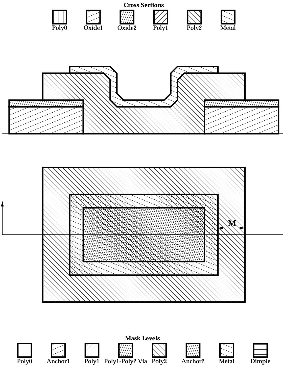
Figure 2.12. M: POLY2 enclose METAL-3.0 \mu\text{m}
