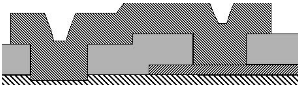
Figure 2.19. Poly 1 properly overlaps ANCHOR1 holes to prevent attack of underlying films as seen in figure 2.18. By completely overlapping the anchor holes, the maximum topography is also reduced (see fig. 1.1 for fill patterns).
