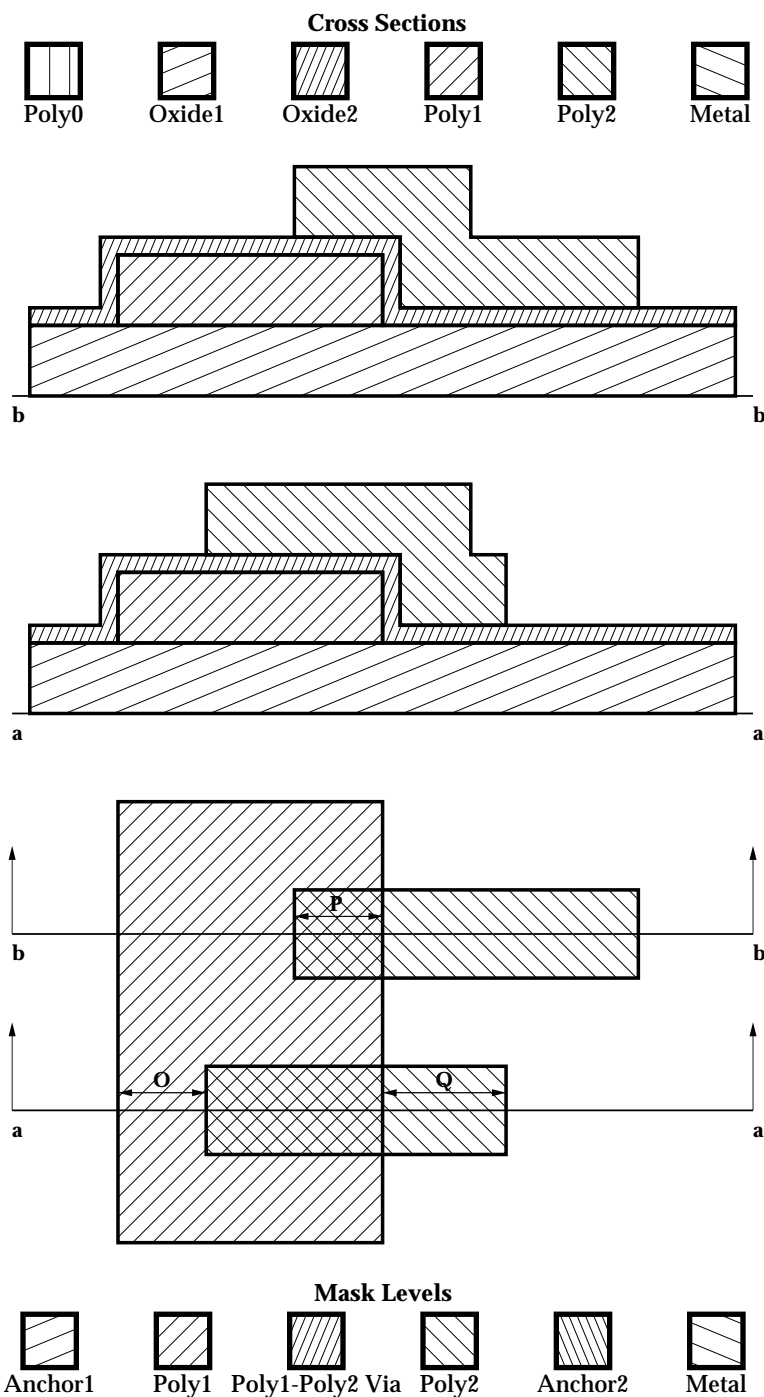
Figure 2.14. P: POLY2 cut-in POLY1–5.0 \mu\text{m}
