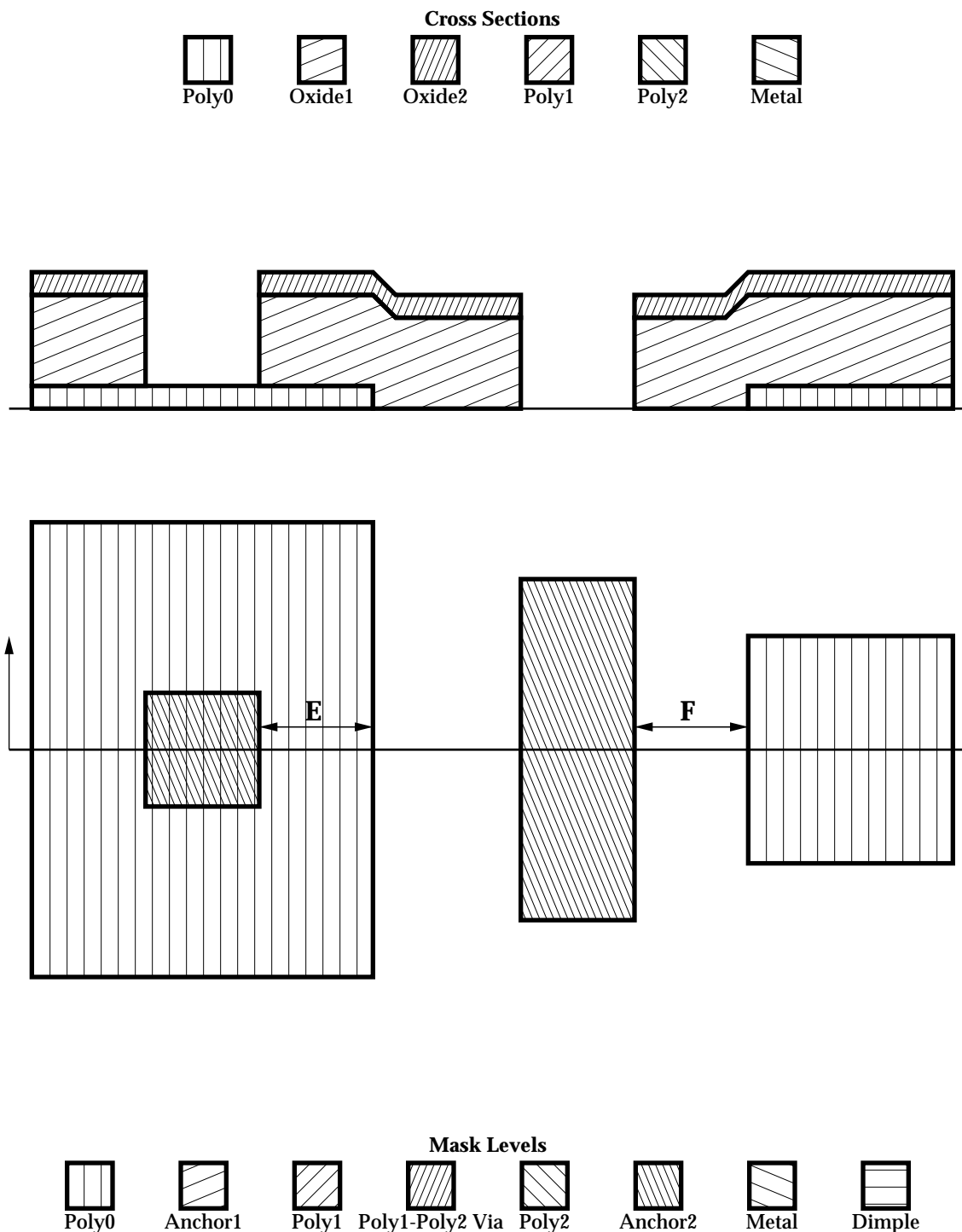
Figure 2.8. E: POLY0 enclose ANCHOR2-5.0 \mu\text{m}
