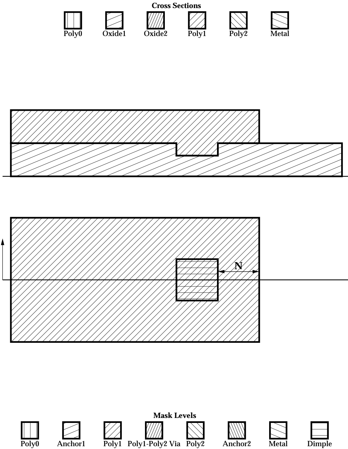
Figure 2.13. N: POLY1 enclose DIMPLE-4.0 μm The amount POLY1 must extend beyond the edge of DIMPLE to ensure the dimple is completely covered by poly 1.
