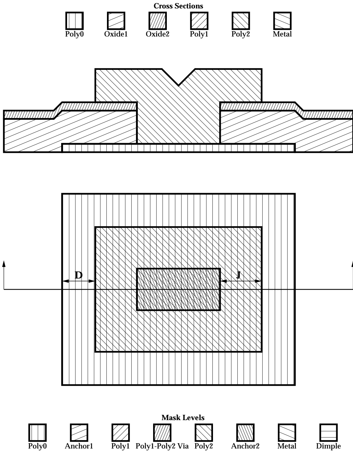
Figure 2.7. O: POLY0 enclose POLY2–5.0 \mu\text{m} The amount Poly 0 must extend beyond the edge of a Poly 2 structure to ensure that Poly 0 is an effective ground plane. J: POLY2 enclose ANCHOR2–5.0 \mu\text{m} The amount Poly 2 must extend beyond an ANCHOR2 hole to ensure complete coverage of the hole.
