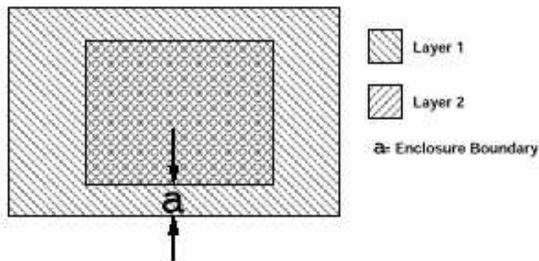
Figure 2.1. Enclose Layer2 by Layer1. a=minimum boundary dimension.
