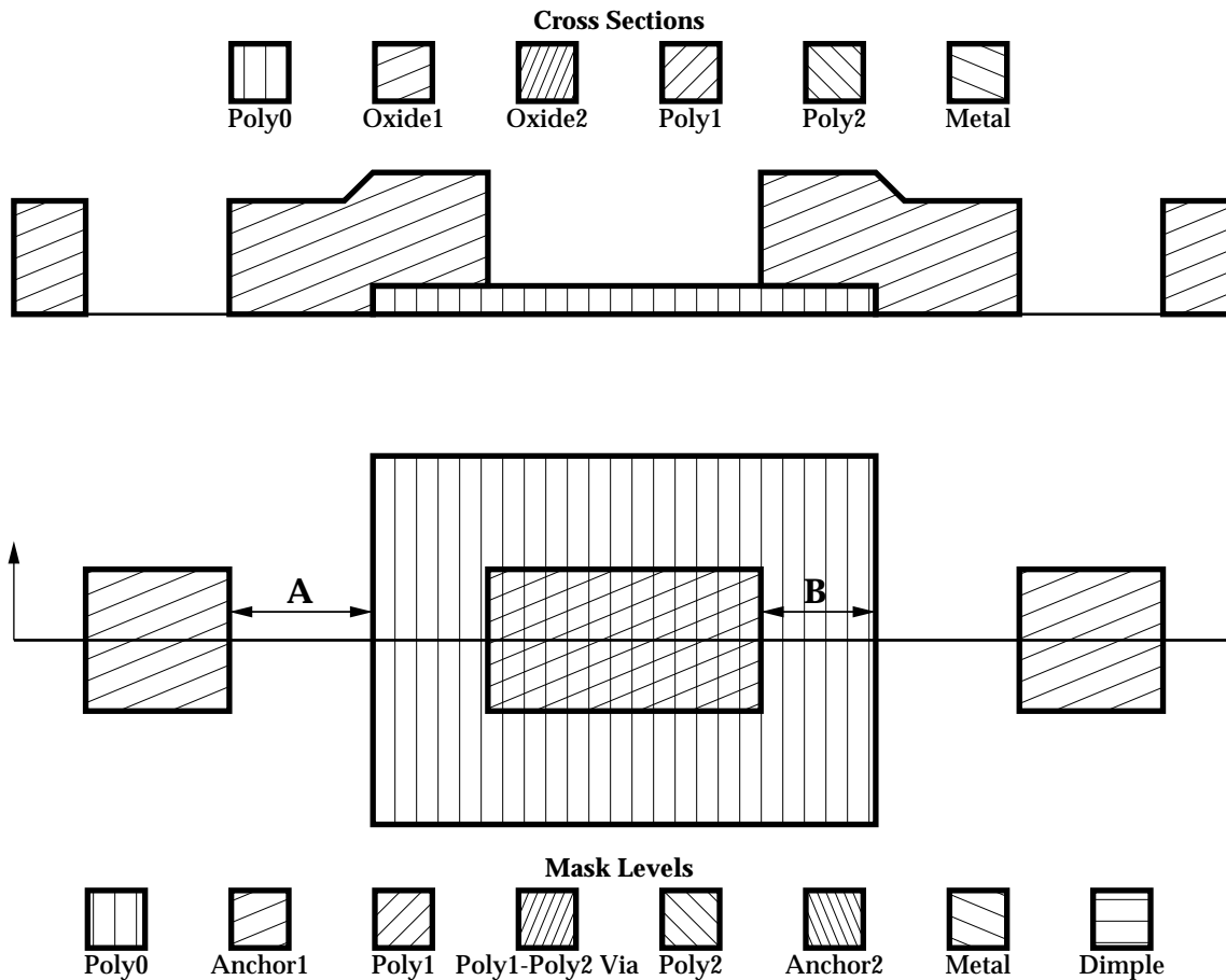
Figure 2.5. A: POLY0 space to ANCHOR1–4.0 μm. The necessary separation between Poly 0 and ANCHOR1 hole to ensure that Poly 0 is not exposed. B: POLY0 enclose ANCHOR1–4.0 μm. The distance necessary between the edge of Poly 0 and an ANCHOR1 hole to ensure the hole does not extend beyond the edge of Poly 0.
