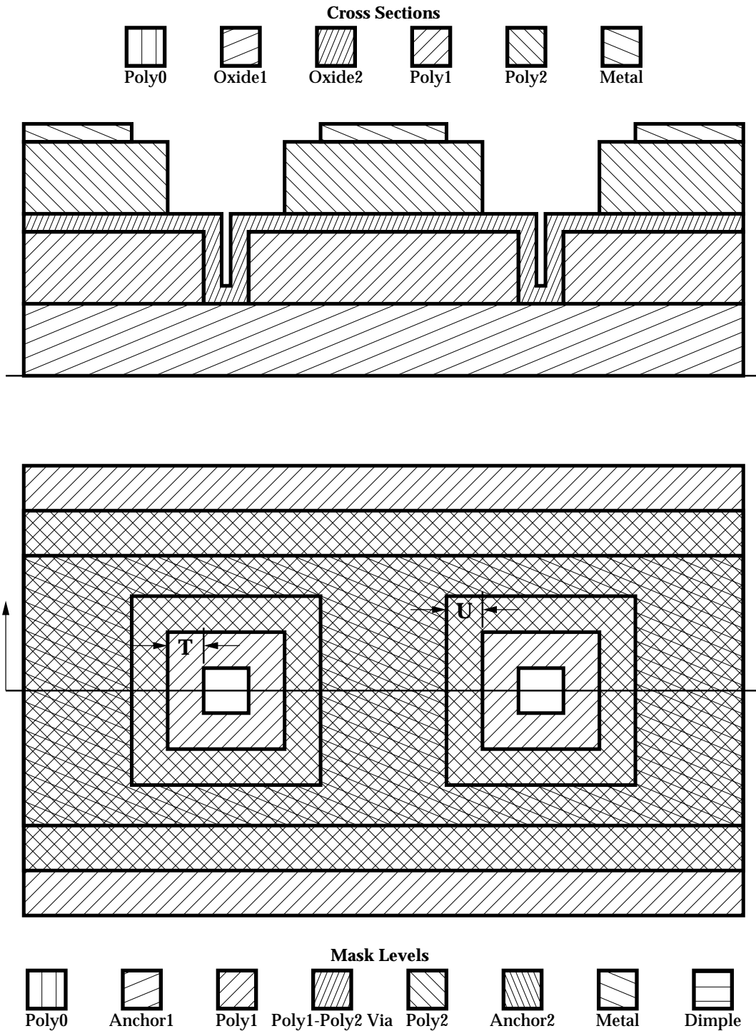
Figure 2.16. T: HOLE2 enclose HOLE1-2.0 \mu\text{m} The necessary border of HOLE2 around HOLE1 to ensure good release results. U: HOLEM enclose HOLE2-2.0 \mu\text{m} The necessary border of HOLEM around HOLE2 to ensure good release results.
