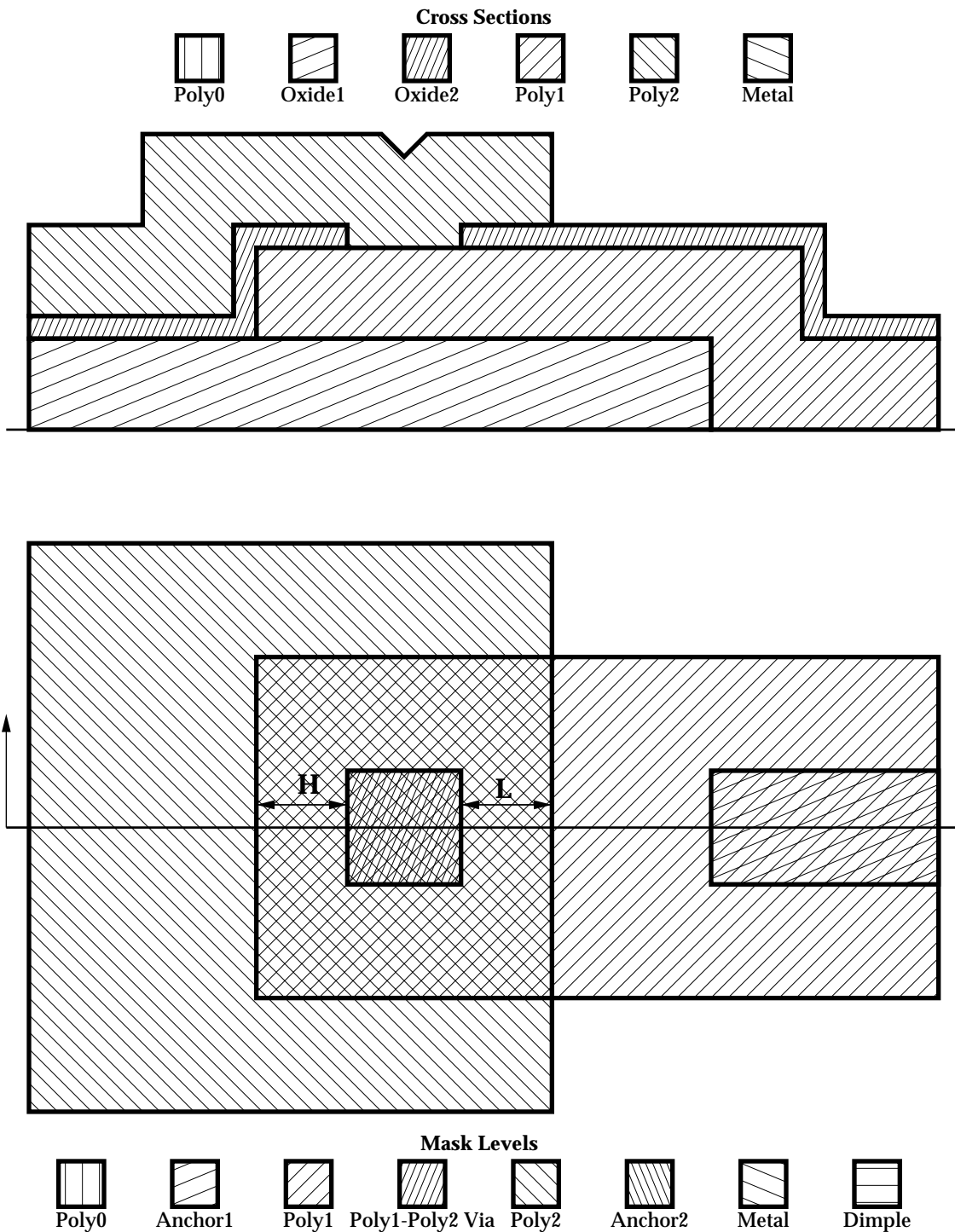
Figure 2.9. H: POLY1 enclose POLY1_POLY2_VIA-4.0 μm The distance between the POLY1_POLY2_VIA hole and the edge of Poly 1 necessary to ensure the via hole is entirely over Poly 1. L: POLY2 enclose POLY1_POLY2_VIA-4.0 μm The amount Poly 2 must extend beyond the POLY1_POLY2_VIA hole to ensure complete coverage of the hole.
