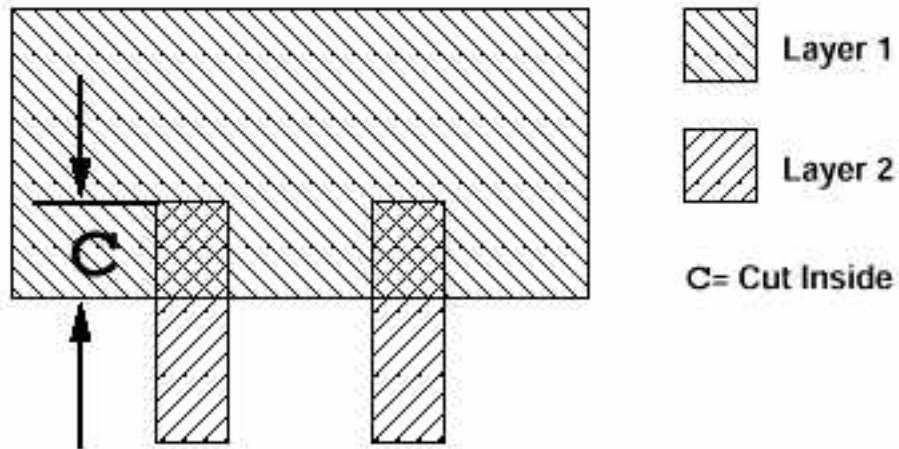
Figure 2.3. Layer1 to Layer2 Cut-in. c=minimum cut-in dimension.
