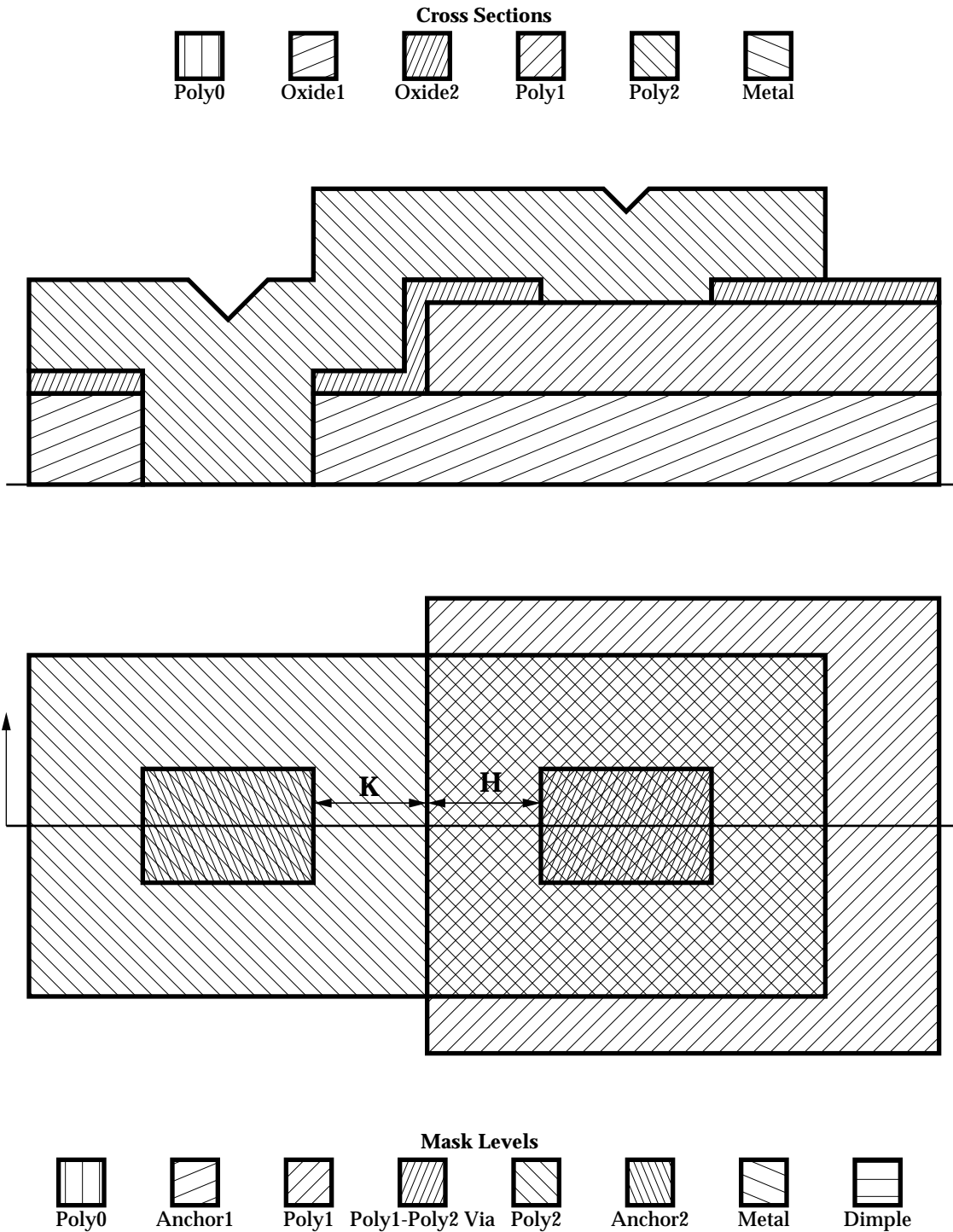
Figure 2.1K: POLY1 space to ANCHOR2–3.0 μm
