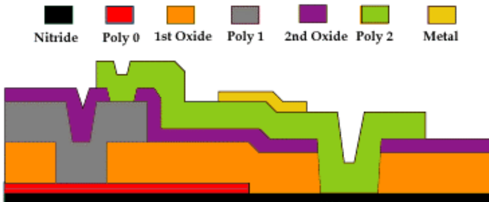
Figure 1.1. Cross sectional view showing all 7 layers of the MUMPs™ process (not to scale).
