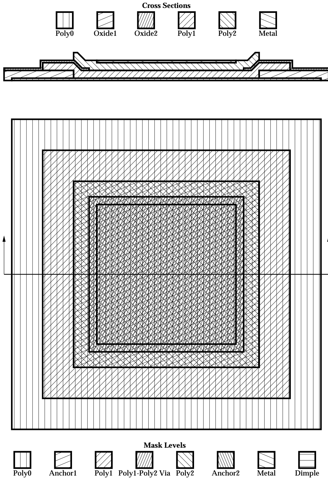
Figure 2.20. Example of proper pad design. The fill patterns from outside to inside are POLY0, POLY1, ANCHOR1 and POLY2 (superimposed), POLY1_POLY2_VIA, and METAL.
