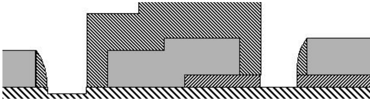
Figure 2.18. Poly 1 does not completely cover ANCHOR1 holes. Much of Nitride has been removed and all of Poly 0 is etched away in exposed area (see fig. 1.1 for fill patterns).
