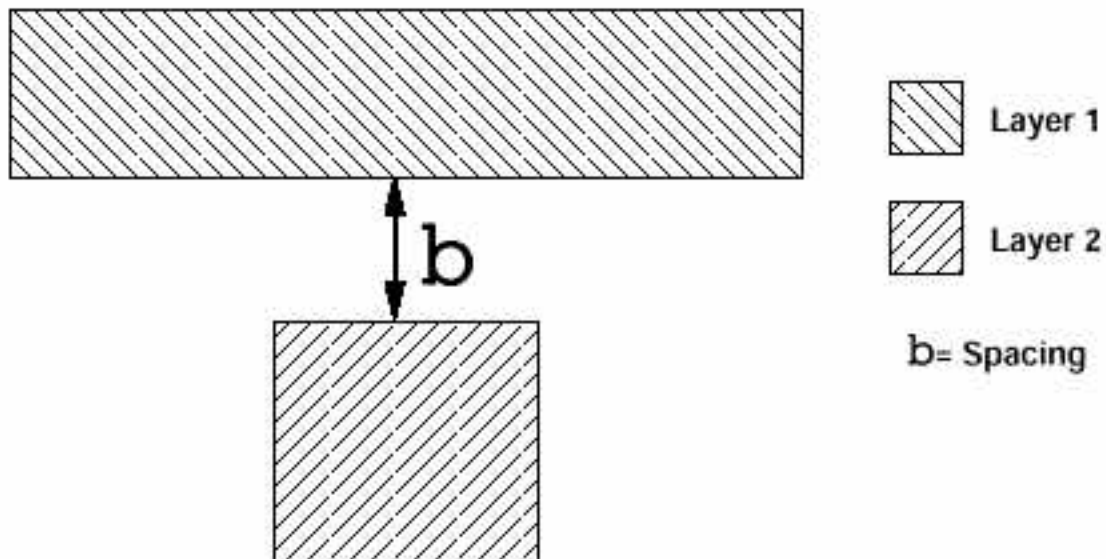
Figure 2.2. Spacing Layer1 to Layer2. b=minimum spacing
