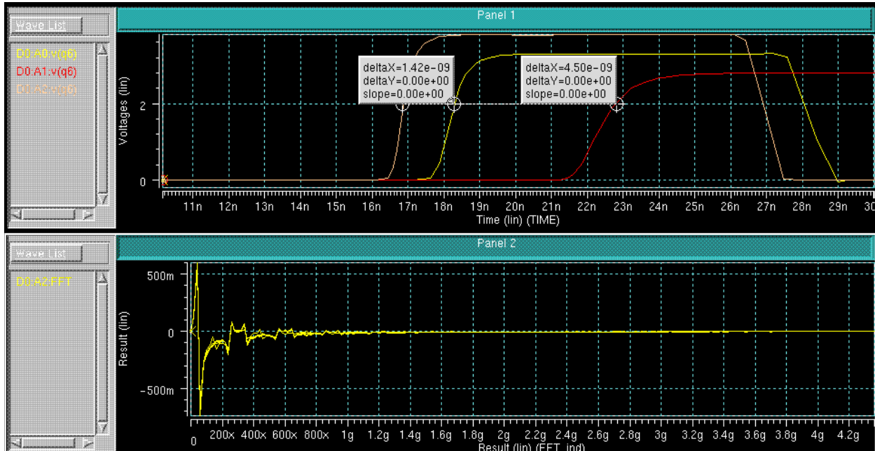
Figure 11-8 Time and frequency response from FFT simulation
